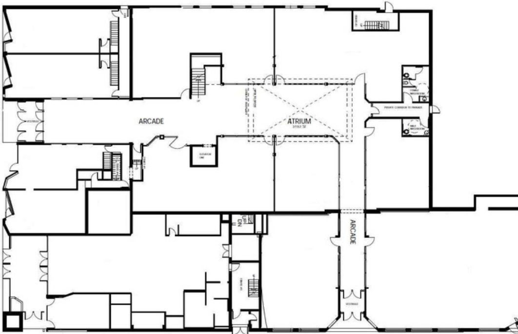
1st Floor
